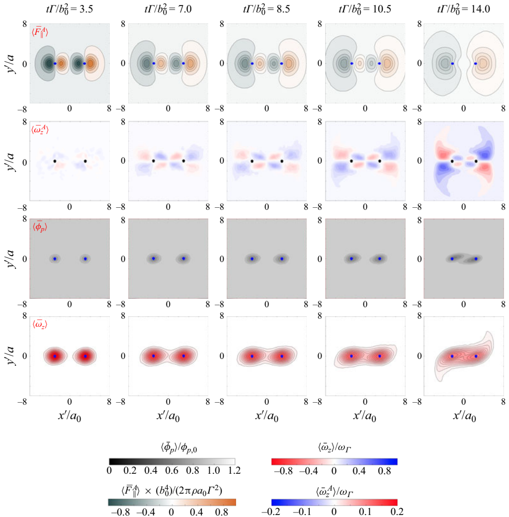
Figure 8. Iso-contours of ensemble-averaged and filtered antisymmetric particle-feedback force along the two vortex centres ( \bar{F}_{\parallel}^A ), antisymmetric axial vorticity ( \langle \bar{\omega}_z^A \rangle ), particle volume fraction ( \bar{\phi}_p ) and total axial vorticity ( \langle \bar{\omega}_z \rangle ) at representative times during the merger. Data correspond to case B with St_{\Gamma} = 0.01 , M = 1 and Re_{\Gamma} = 530 .
