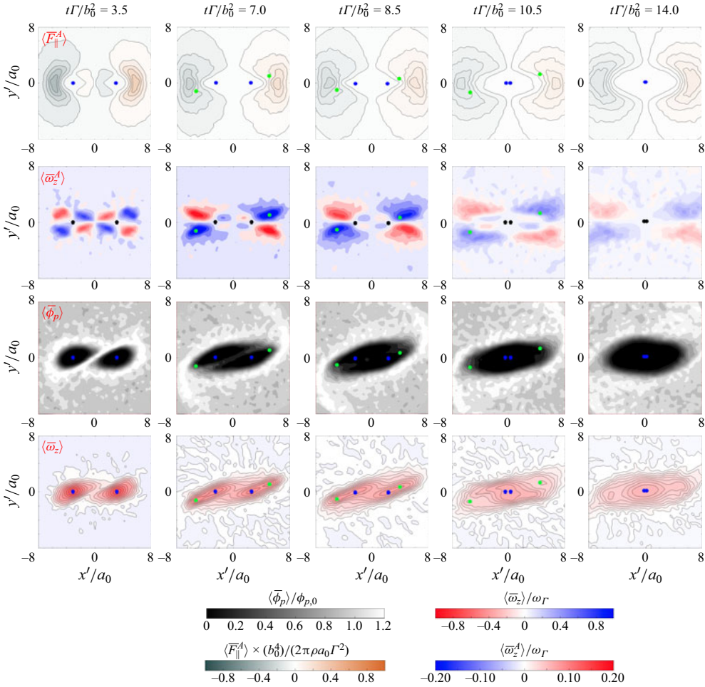
Figure 10. Iso-contours of ensemble-averaged and filtered antisymmetric particle-feedback force along the two vortex centres \langle \bar{F}_\parallel^A \rangle , antisymmetric axial vorticity \langle \bar{\omega}_z^A \rangle , particle volume fraction \langle \phi_p \rangle and total axial vorticity \langle \bar{\omega}_z \rangle at representative times during the merger. Data correspond to case F with St_\Gamma = 0.2 , M = 1 and Re_\Gamma = 530 .
