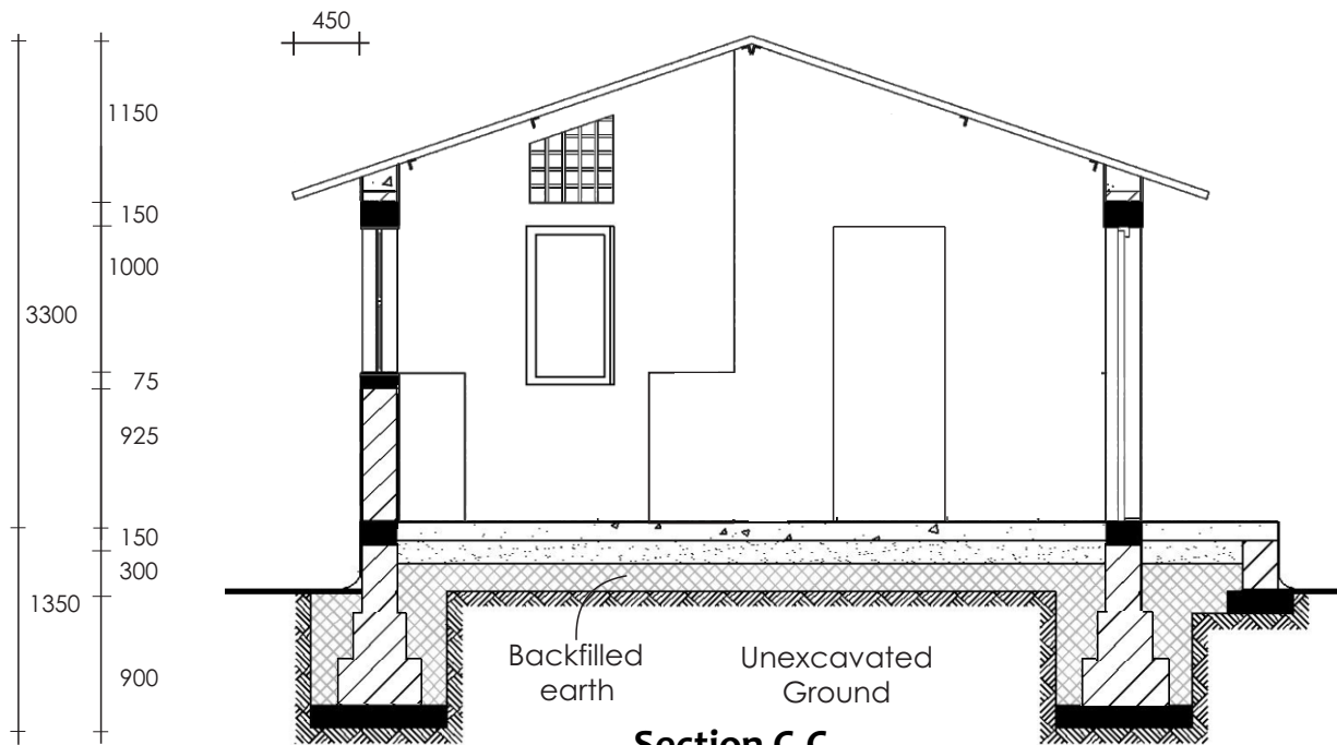
Section C-C
