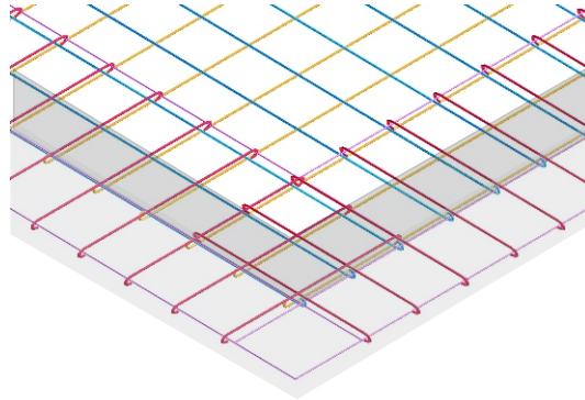
Reinforcement at Slab Corner Edge
