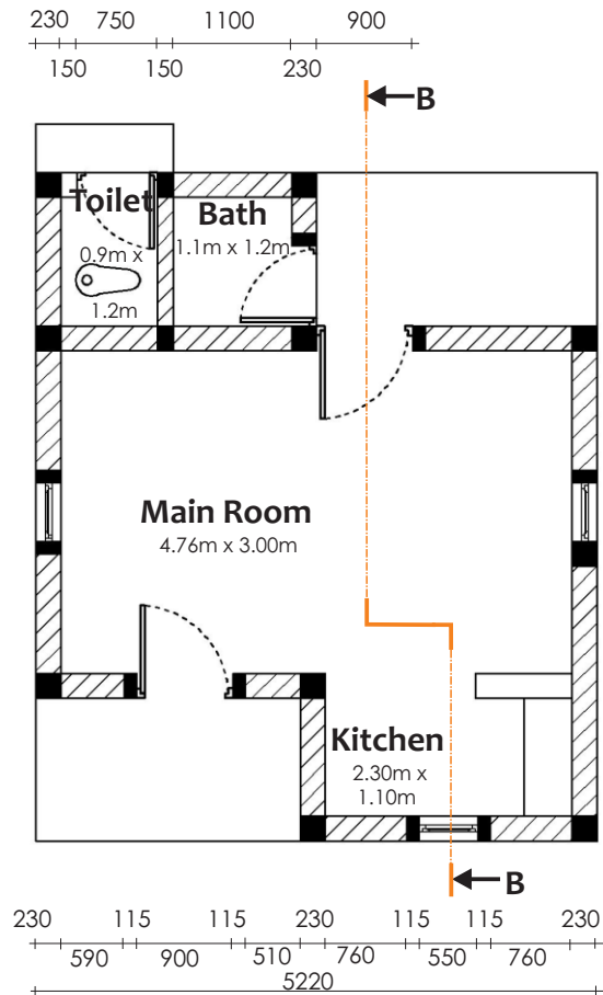
Plan
