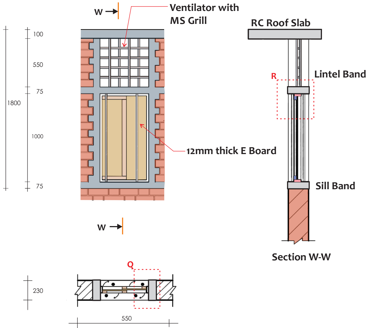
Window Details
