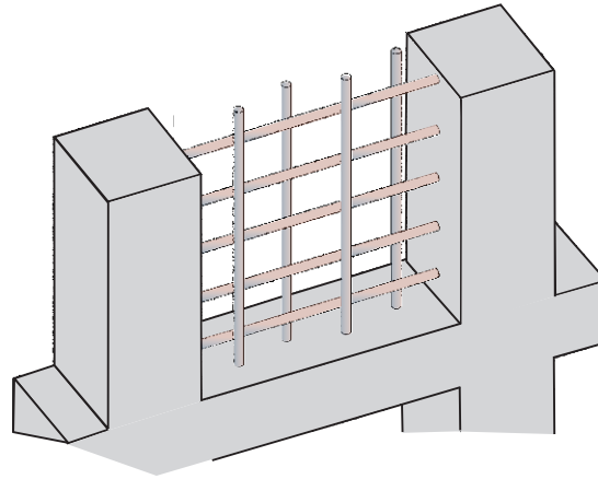
Ventilator with Built-in Steel Grill
