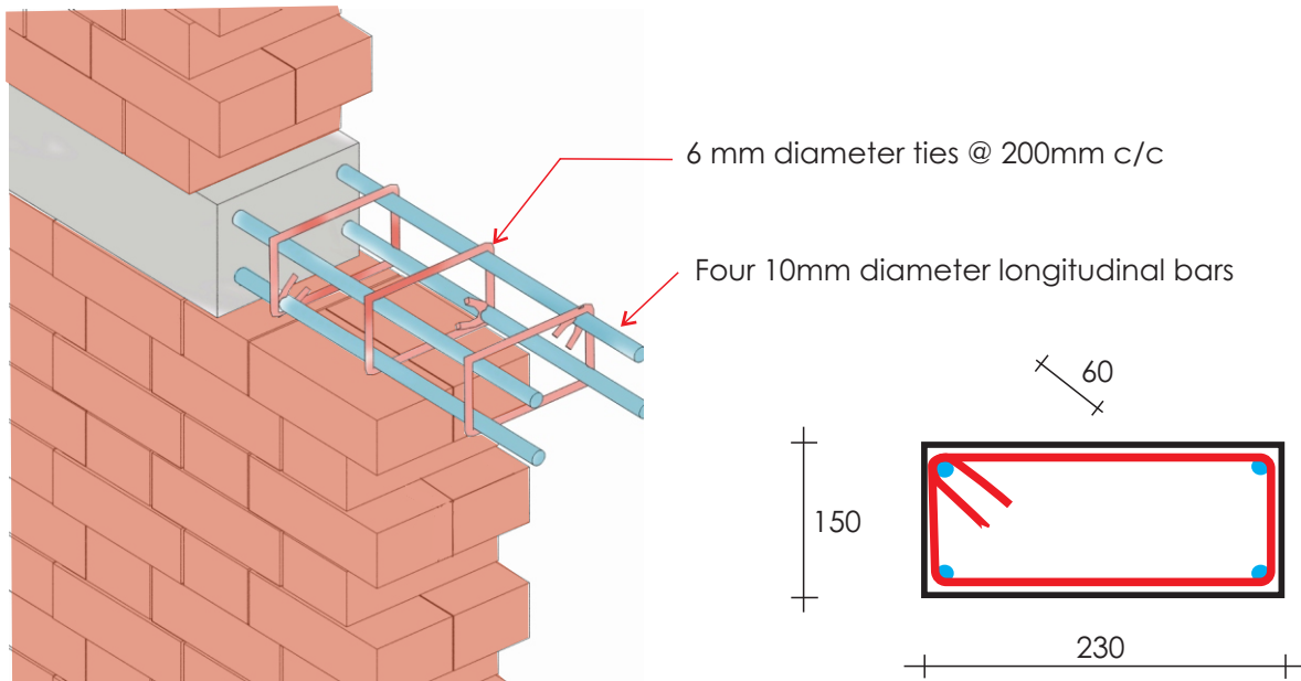
Plinth Band
