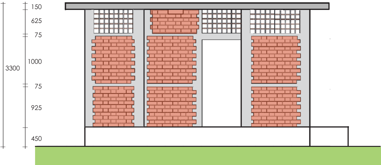
Left Elevation
